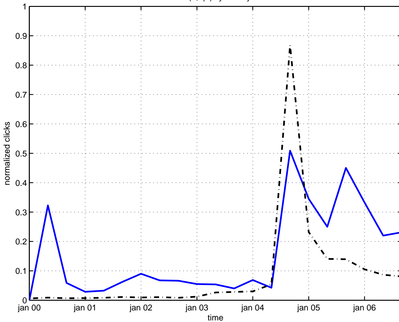
su(1,1|2) symmetry
