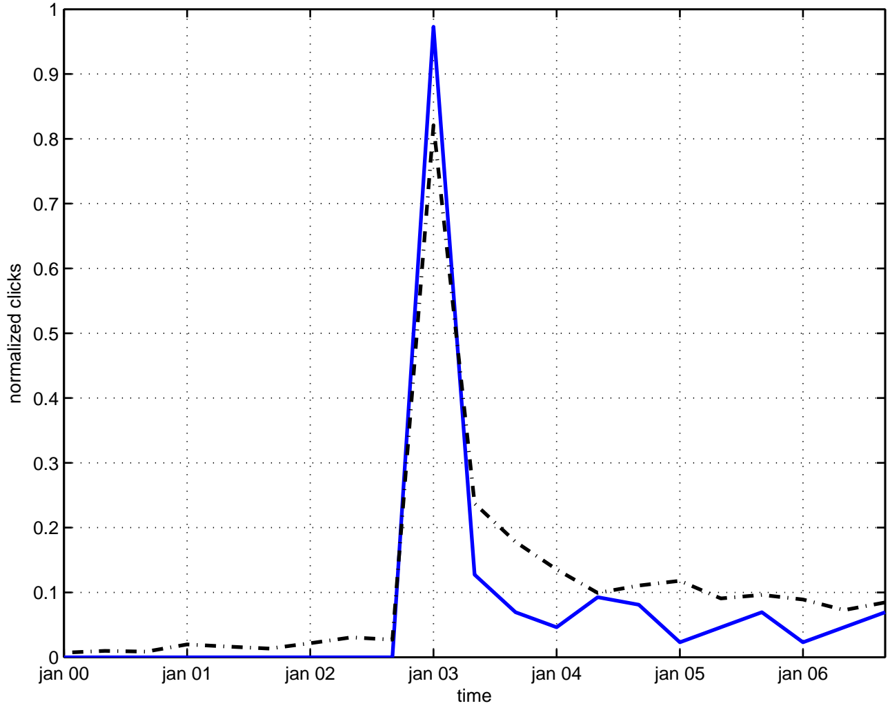
su(1,1|2) invariance
