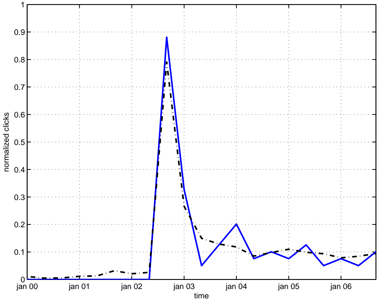
stueckelberg equation
