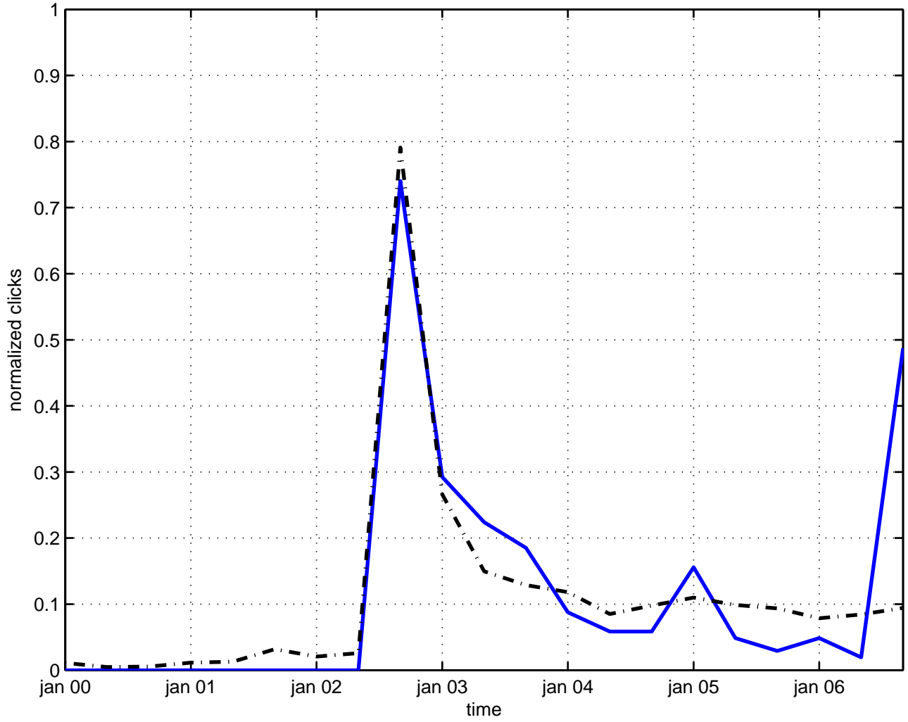
strong interaction pi
