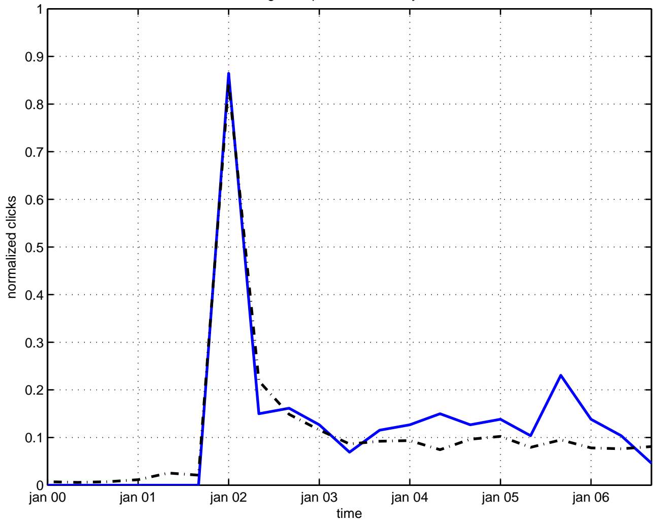
strong field quantum electrodynamics
