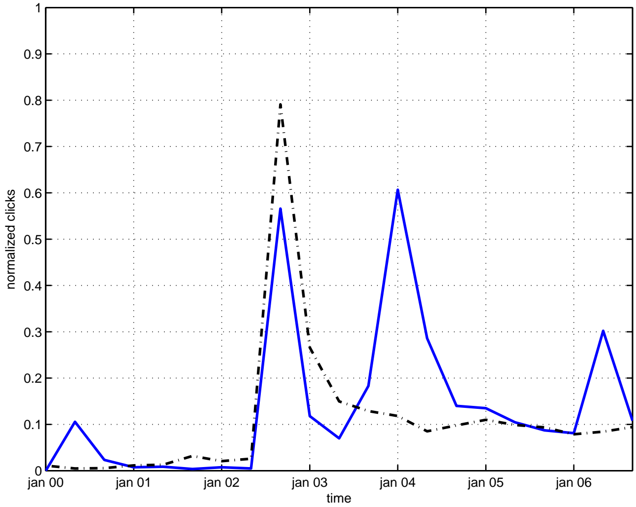
strong field approximation
