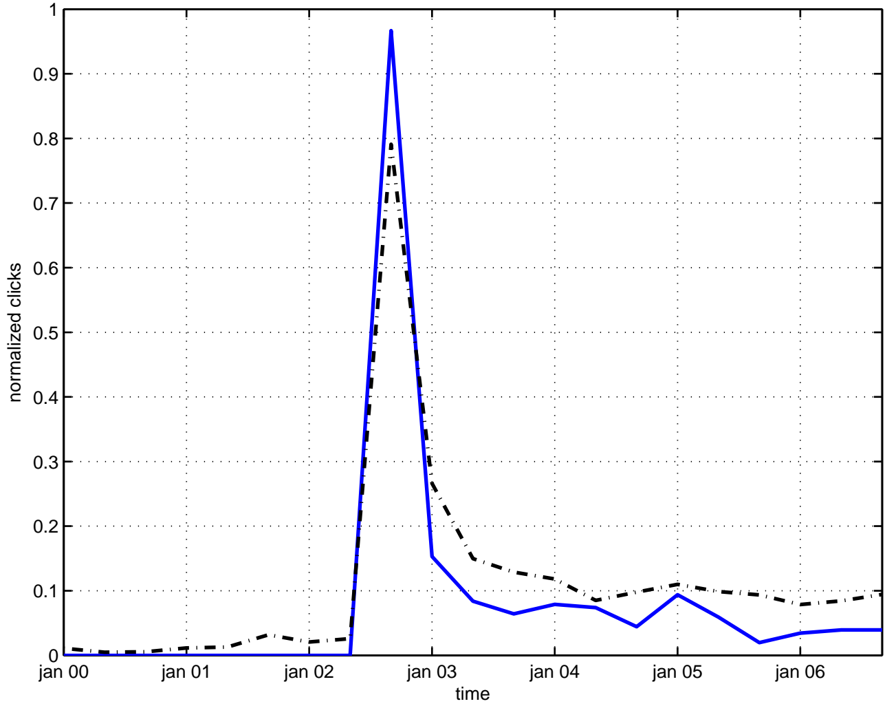
strong coupling quantum chromodynamics
