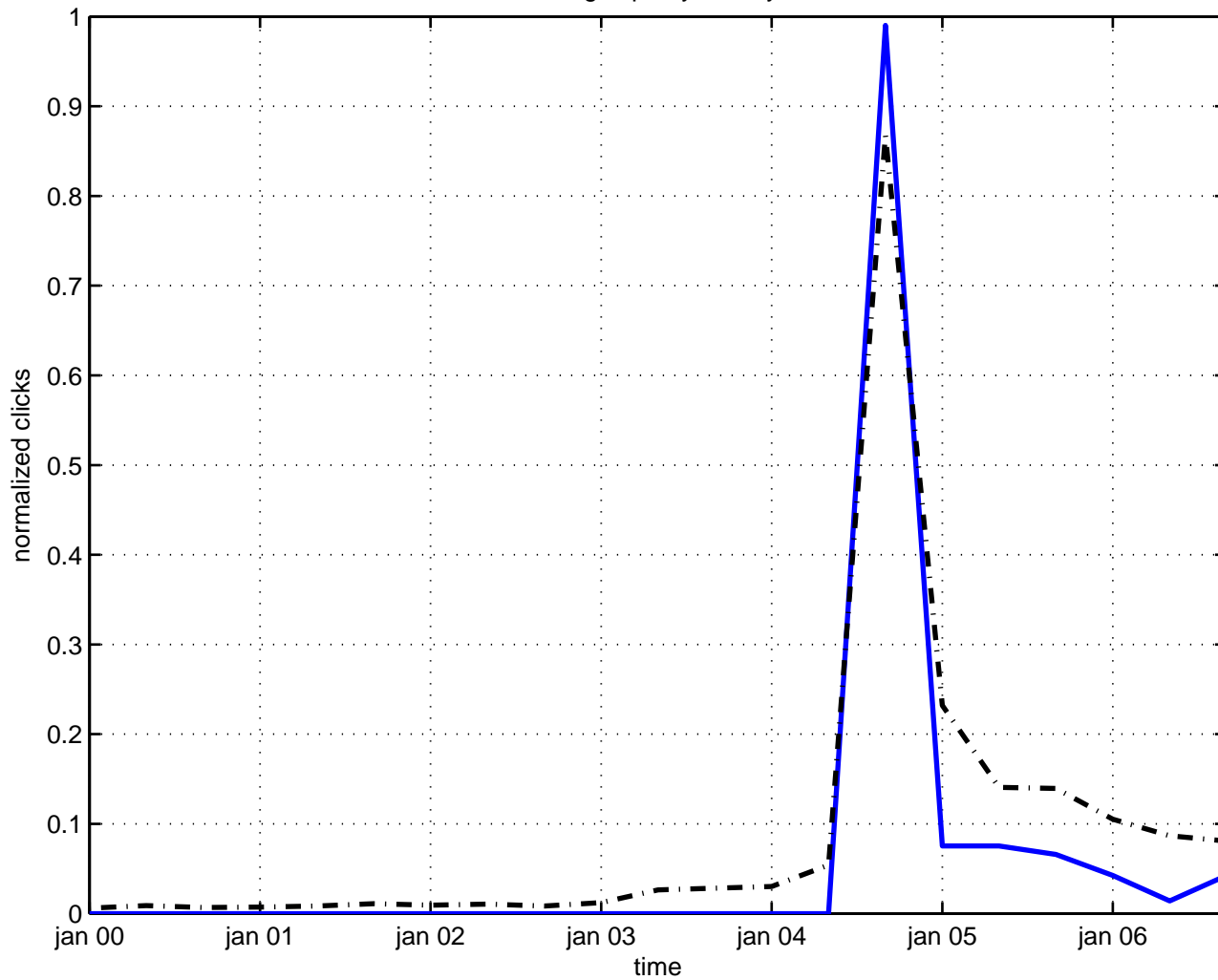
string supersymmetry
