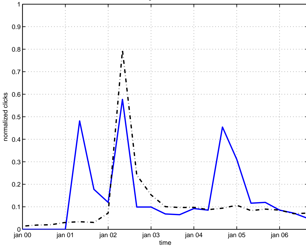
string model fermion
