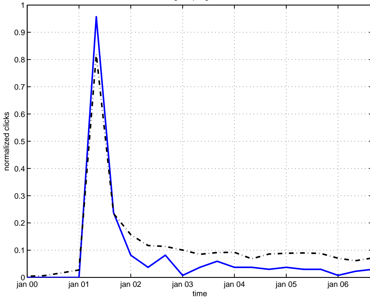
string coupling constant
