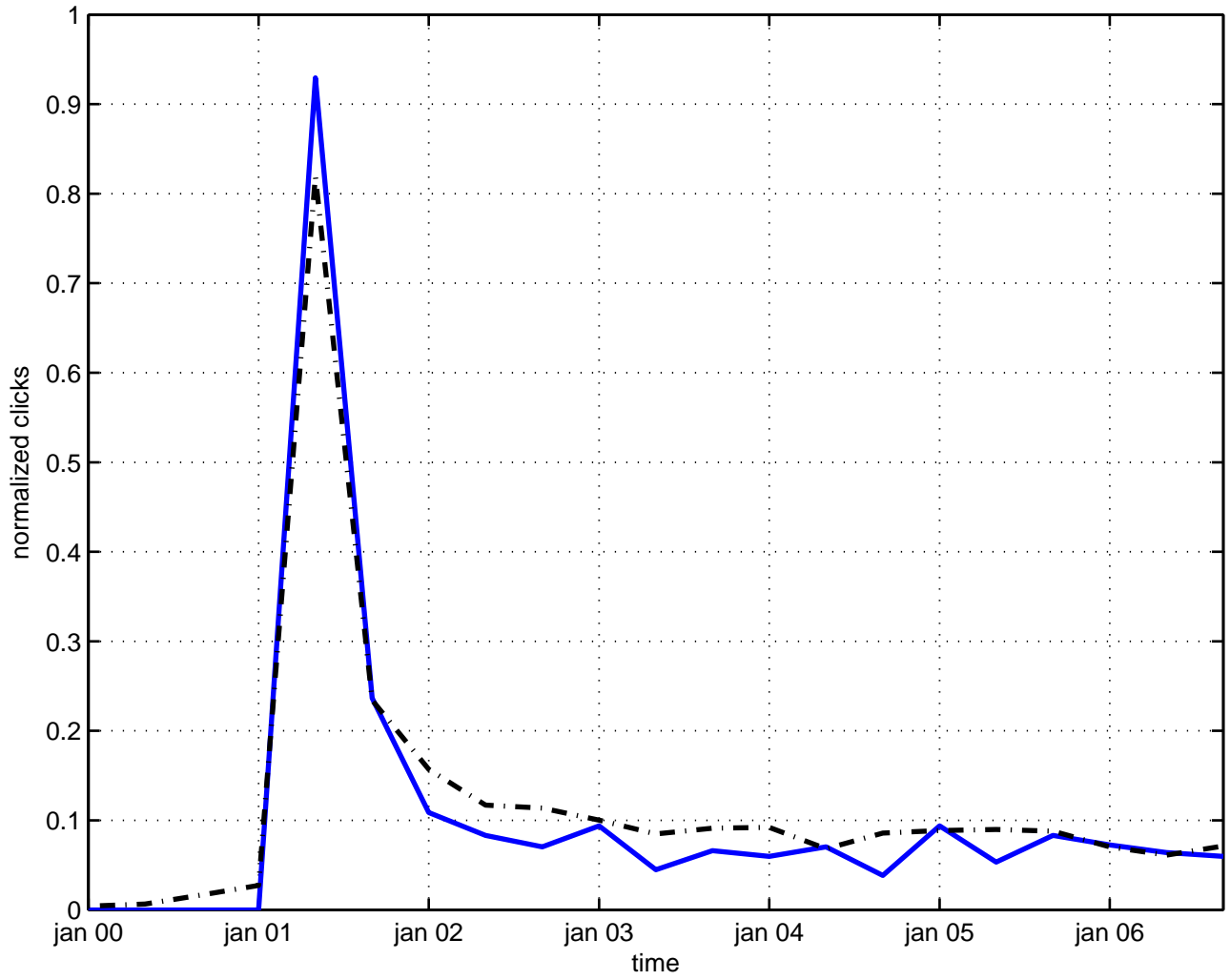
string charge
