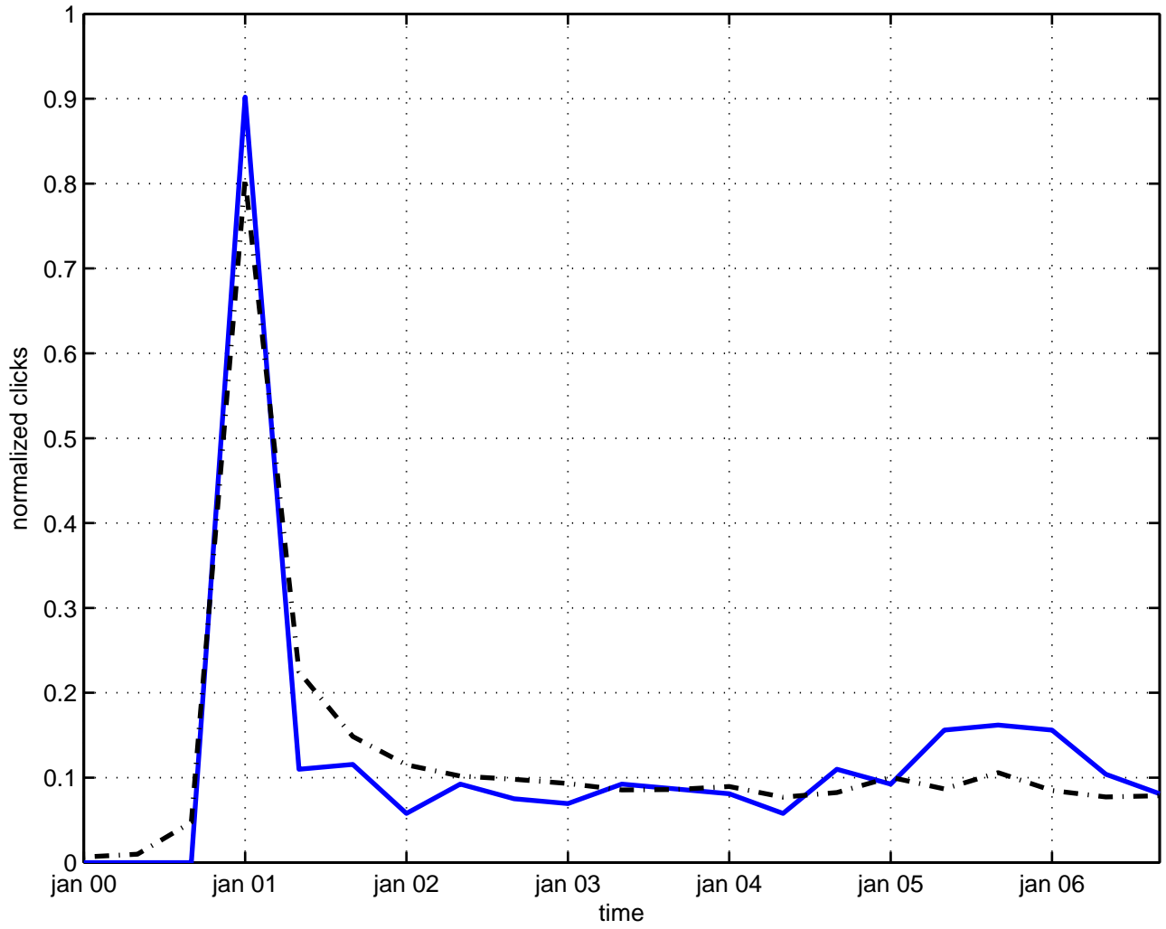
storage ring electron
