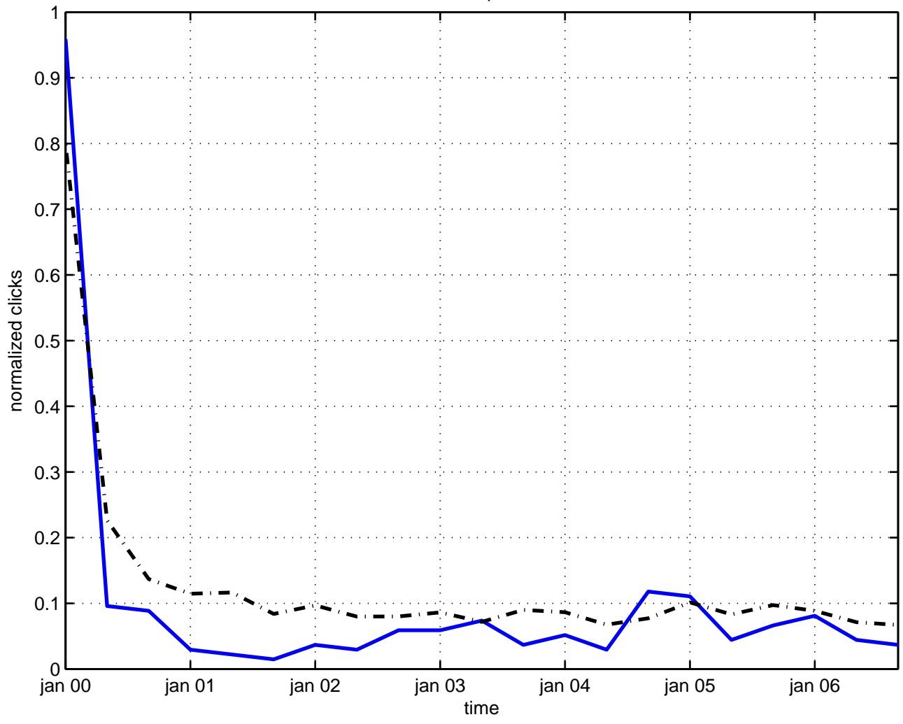
stochastic space-time
