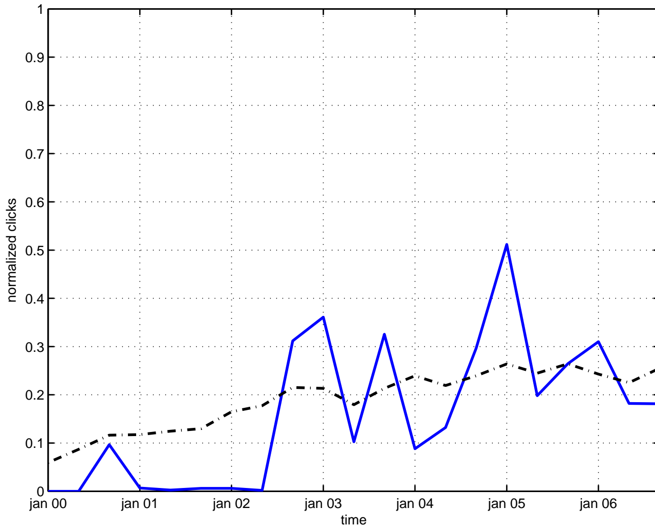
stochastic mathematical methods
