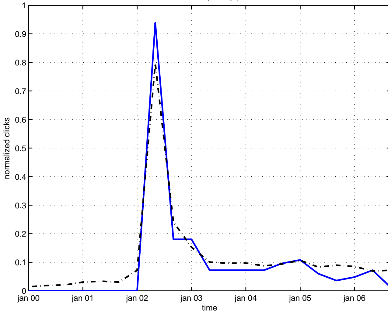
stochastic many-body problem
