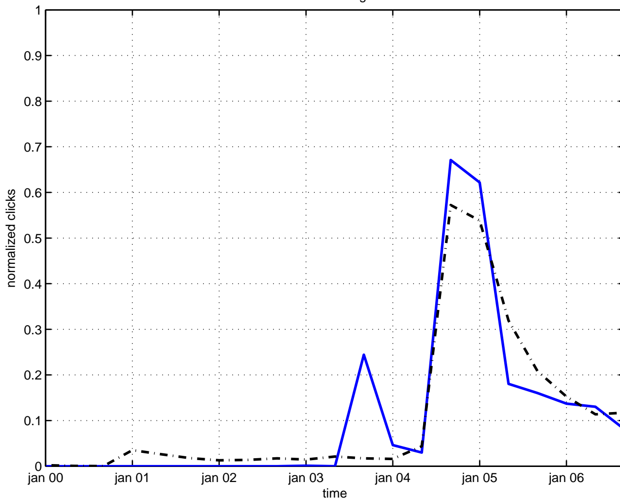
stochastic background
