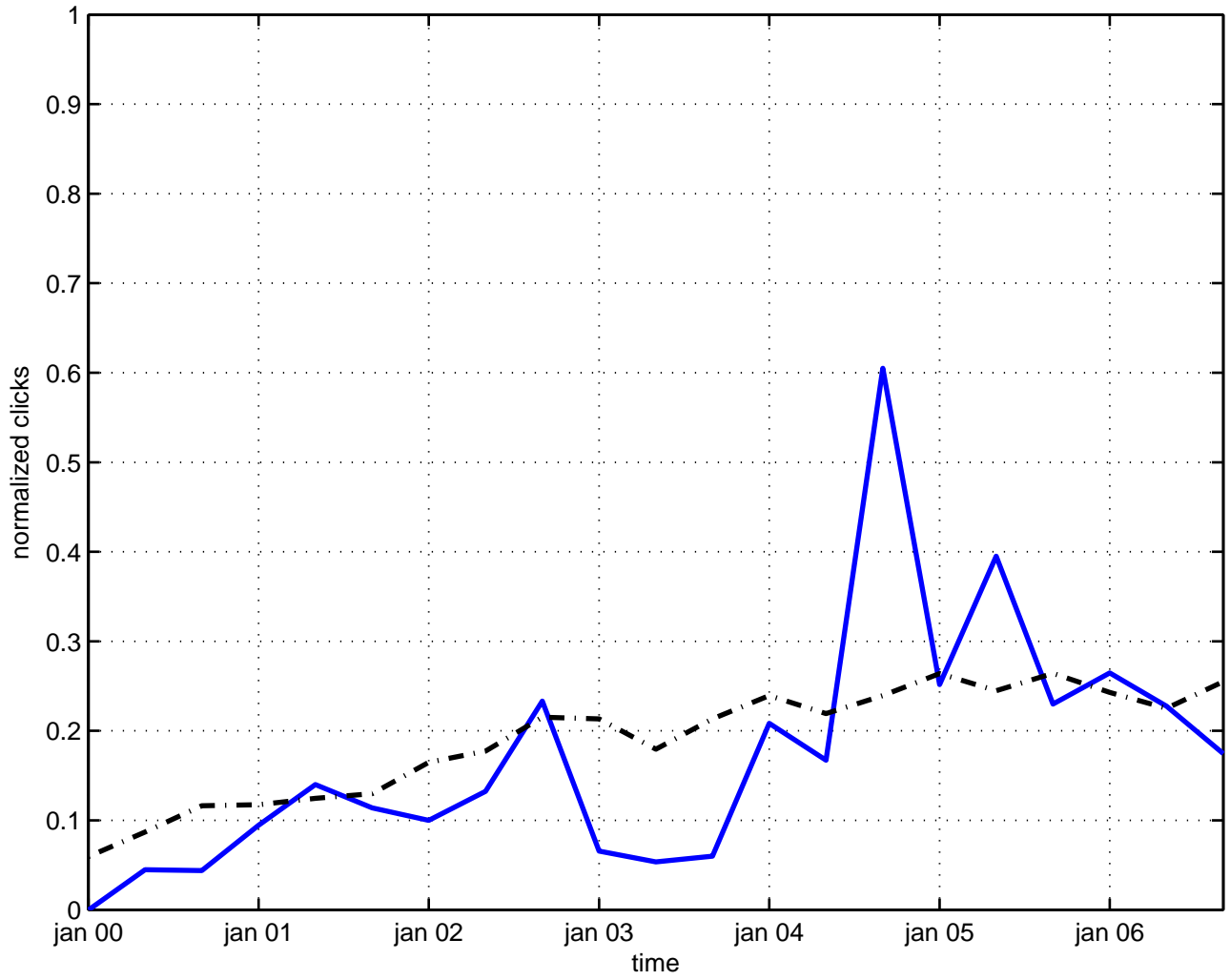
statistics spin
