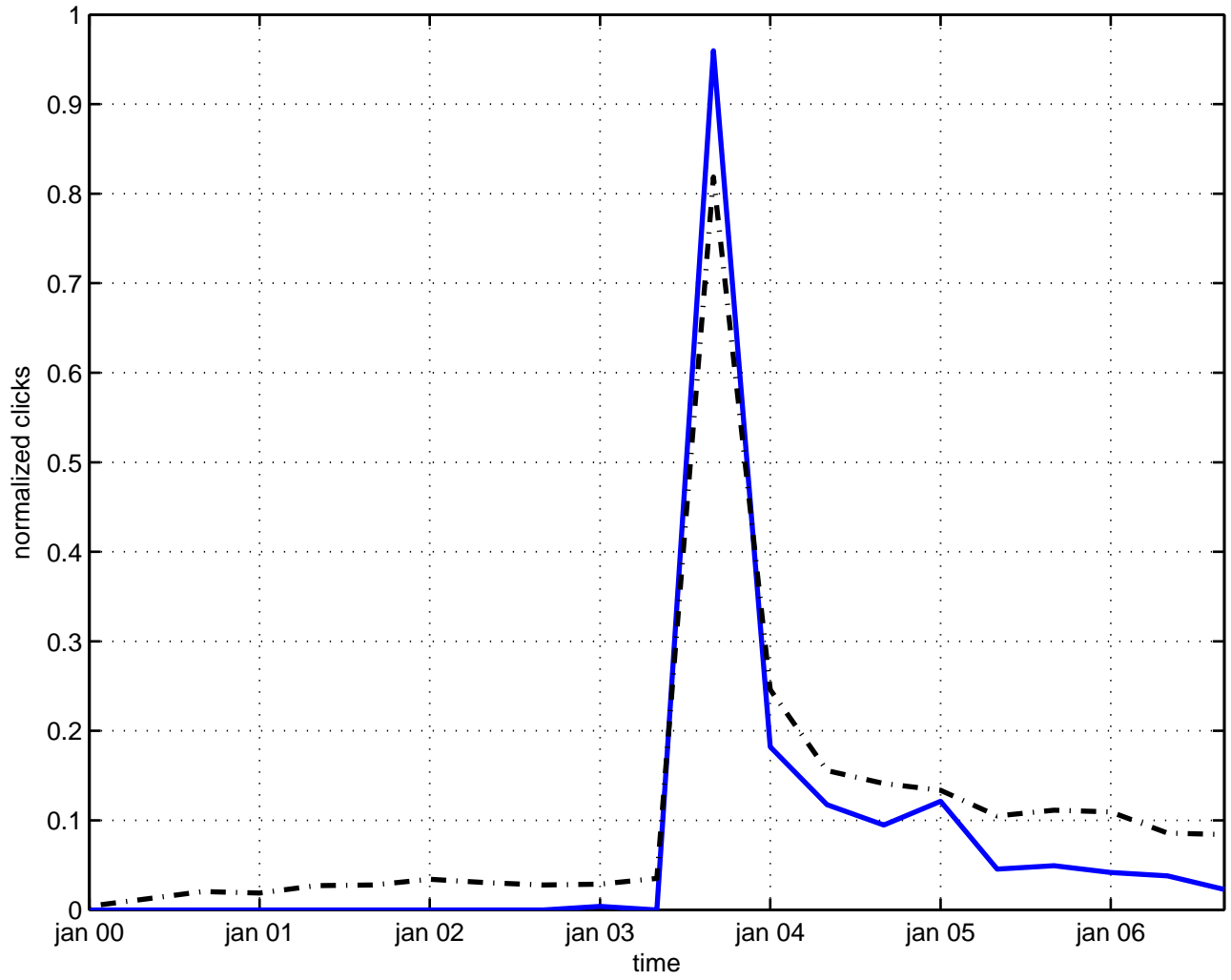
statistics perturbation
