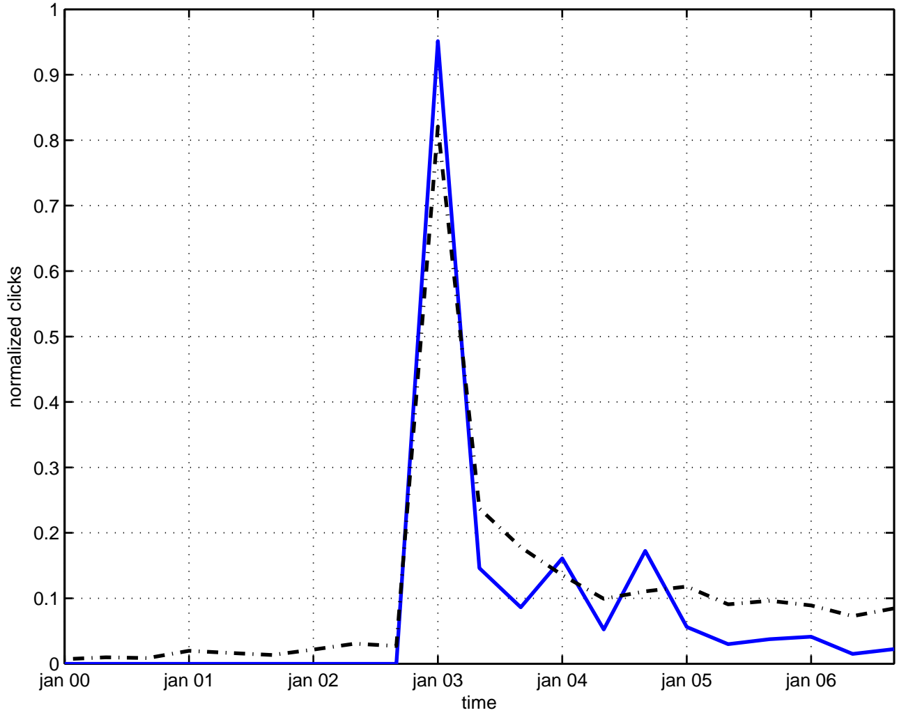
statistical quantum mechanics
