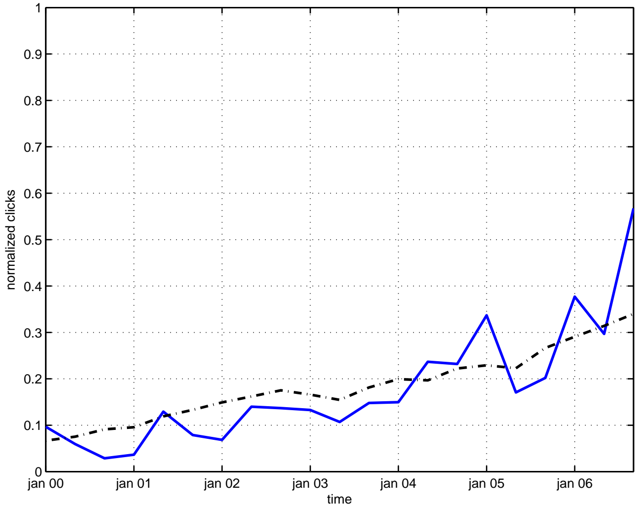
statistical mechanics
