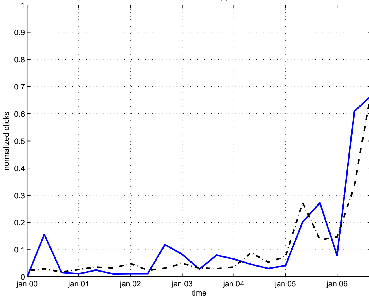
statistical entropy
