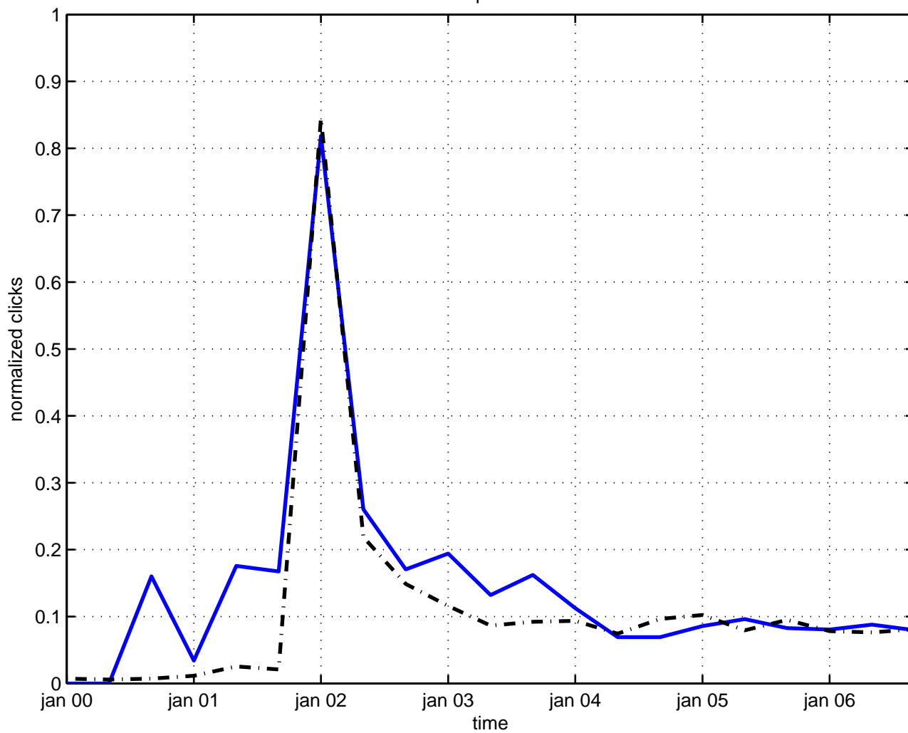
static space-time
