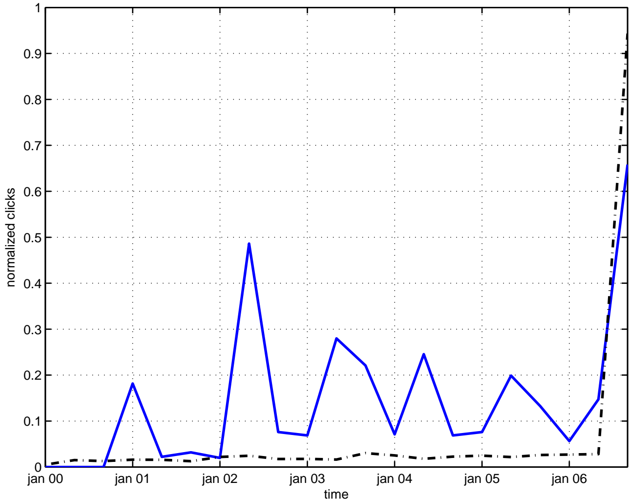
static potential
