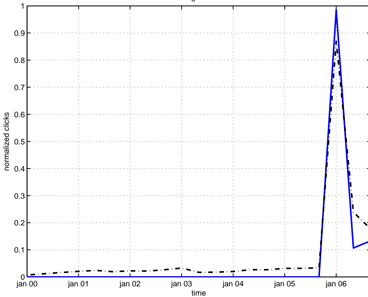
static gravitation
