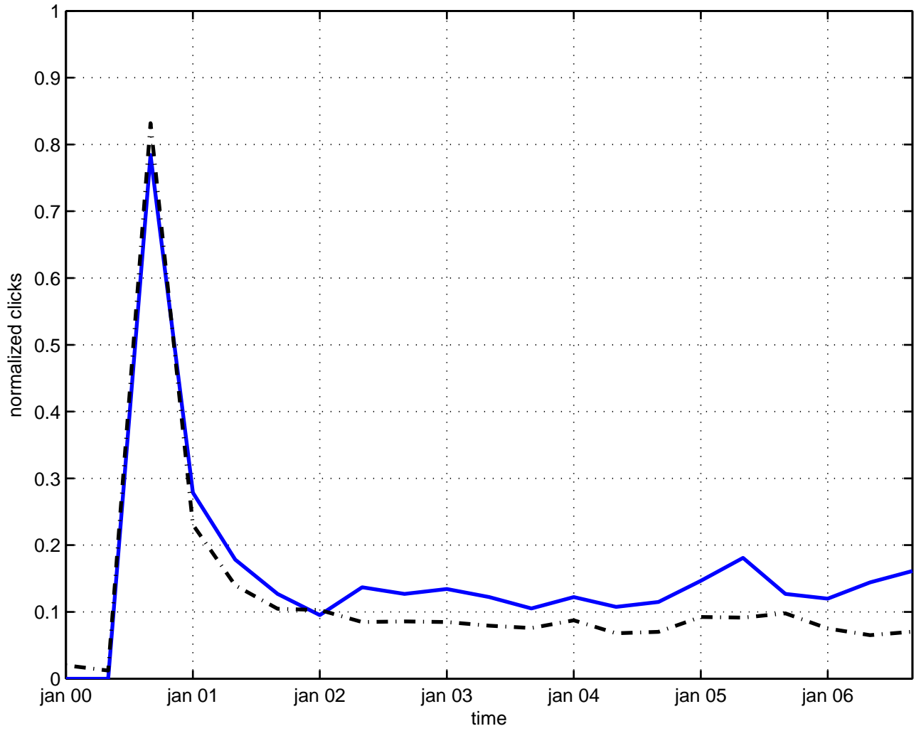
stark effect
