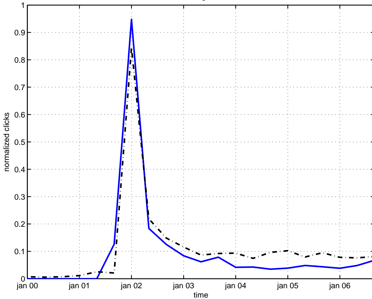
star algebra
