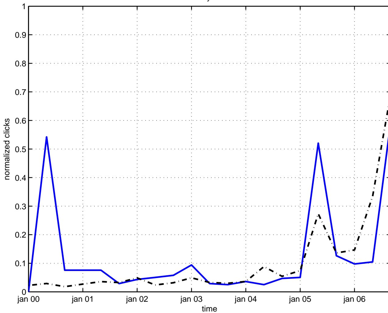
stability vortex
