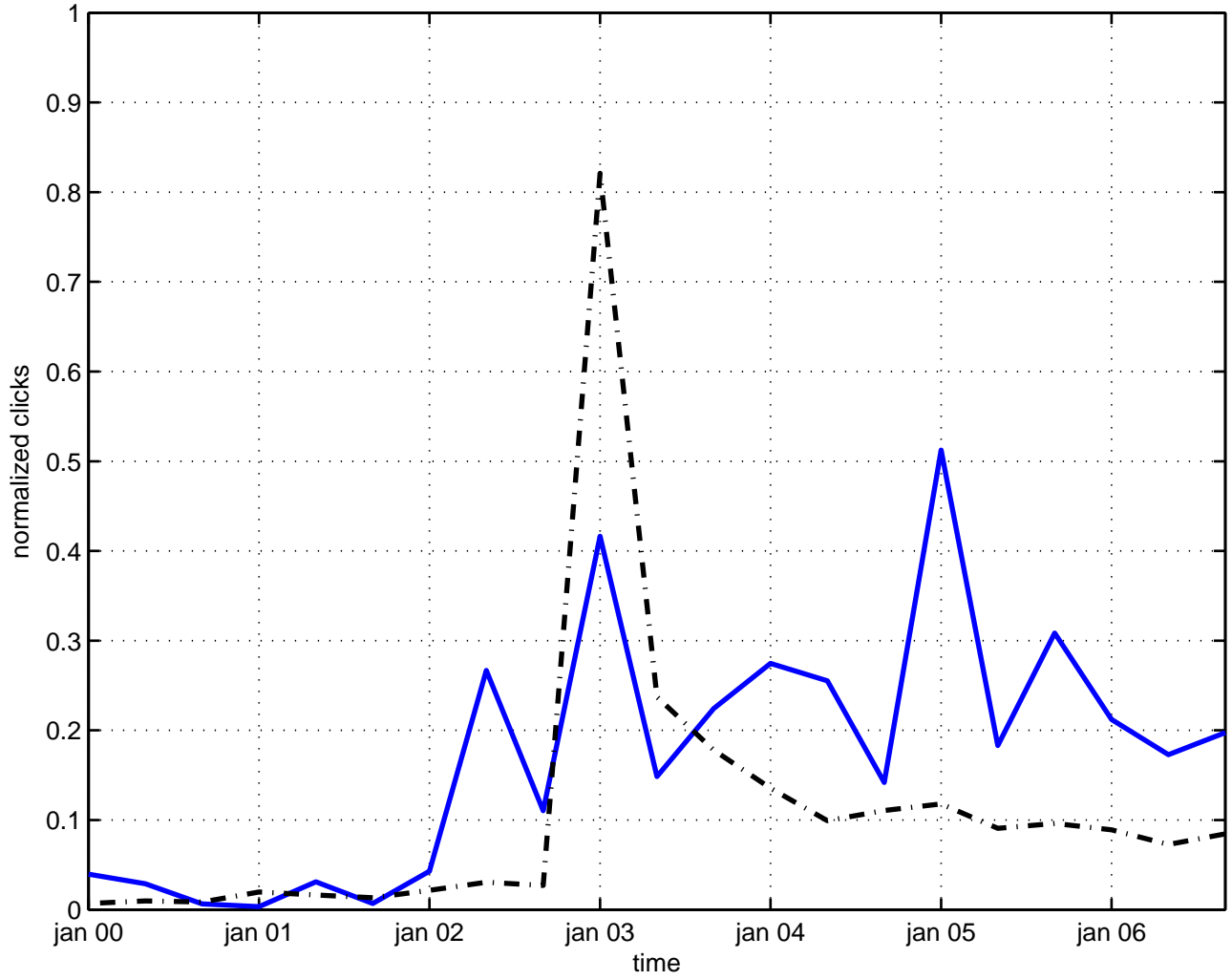
stability space-time
