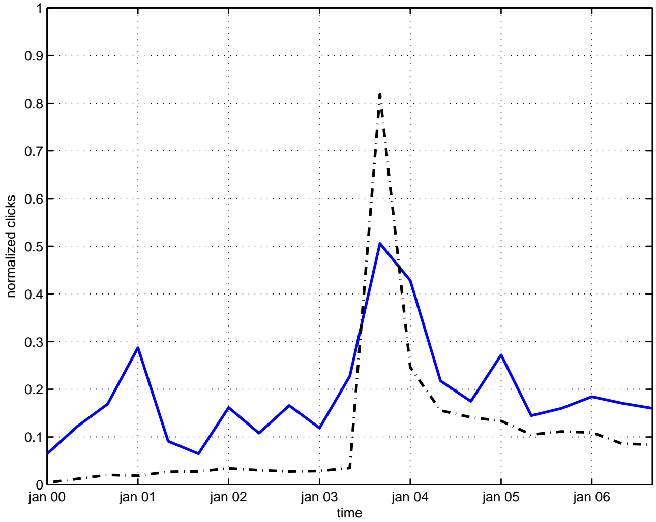
stability radion
