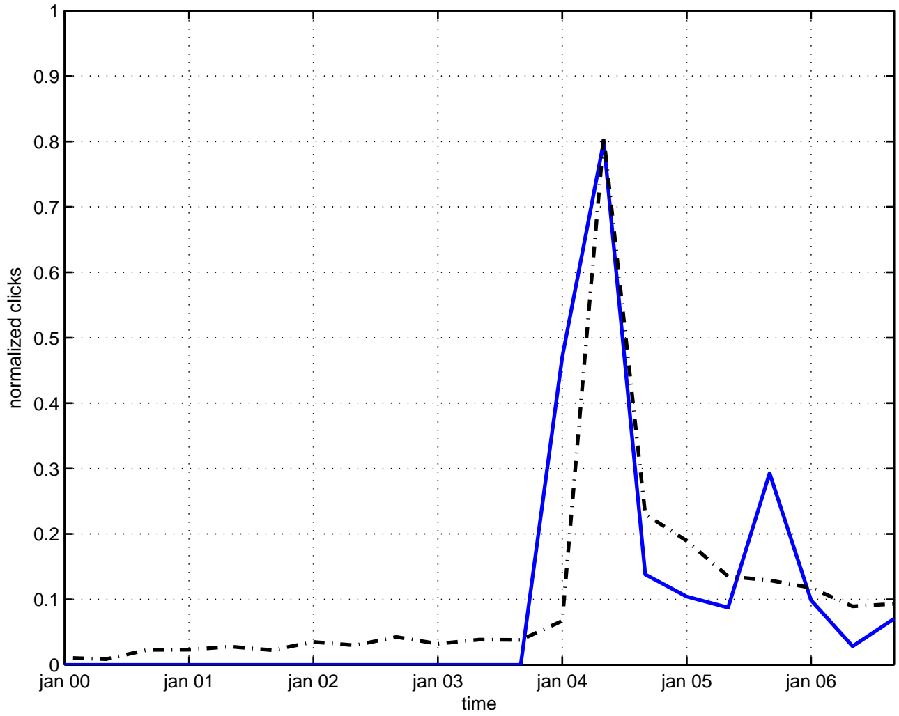
stability quantum gravity
