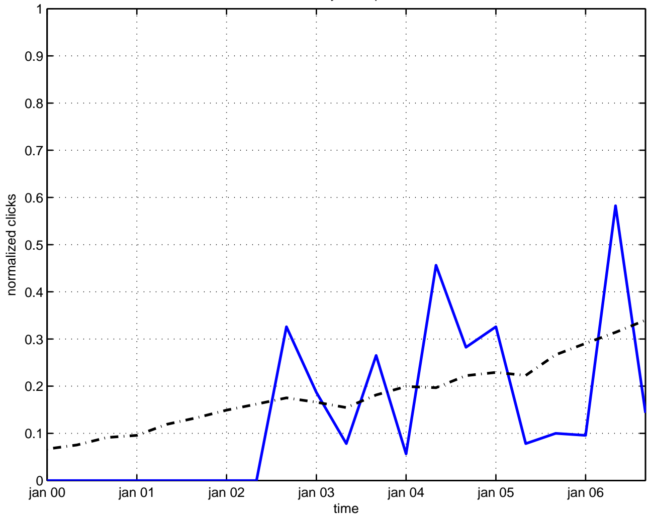
stability monopole
