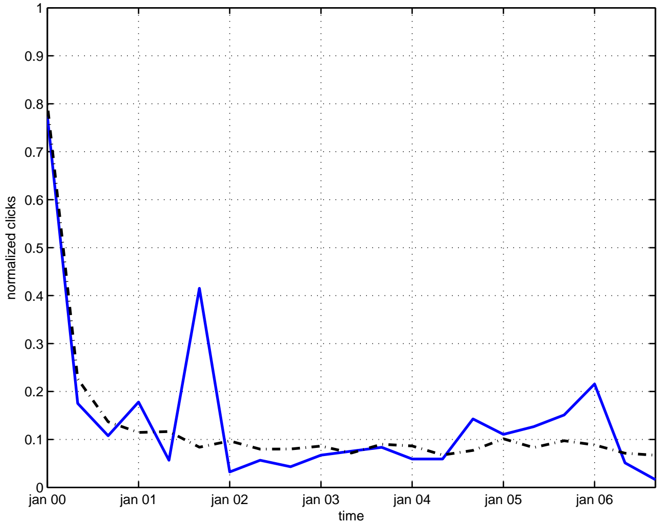
stability graviton
