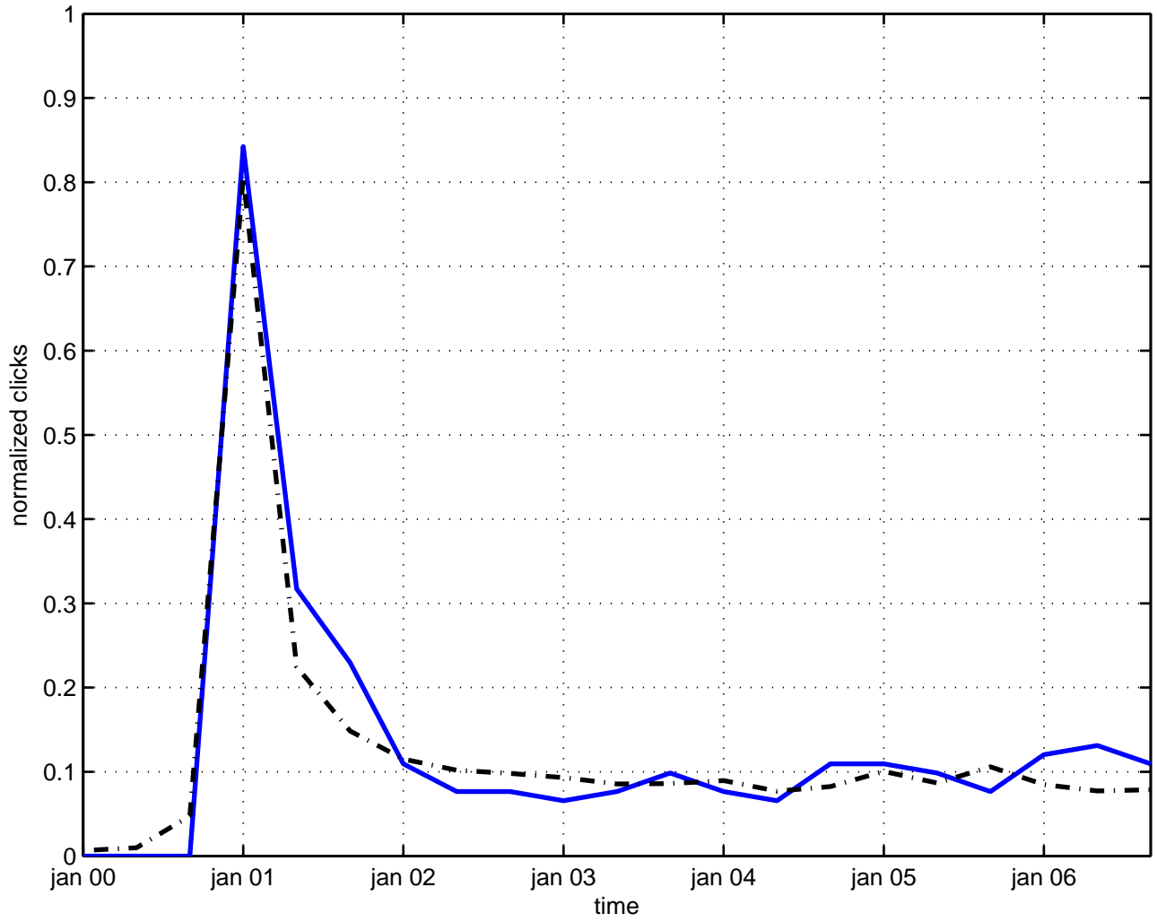
stability gap
