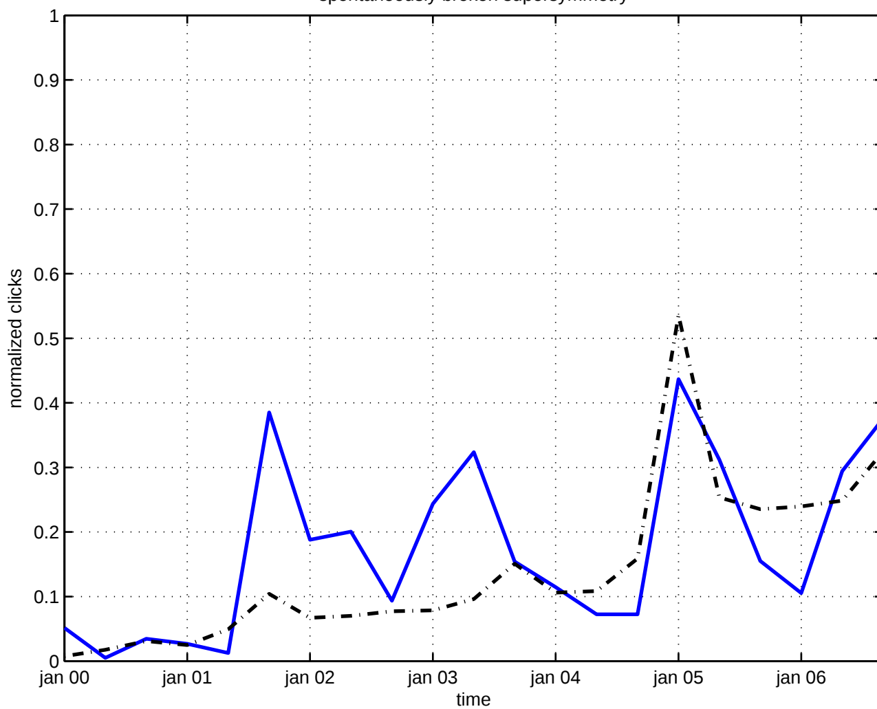
spontaneously broken supersymmetry
