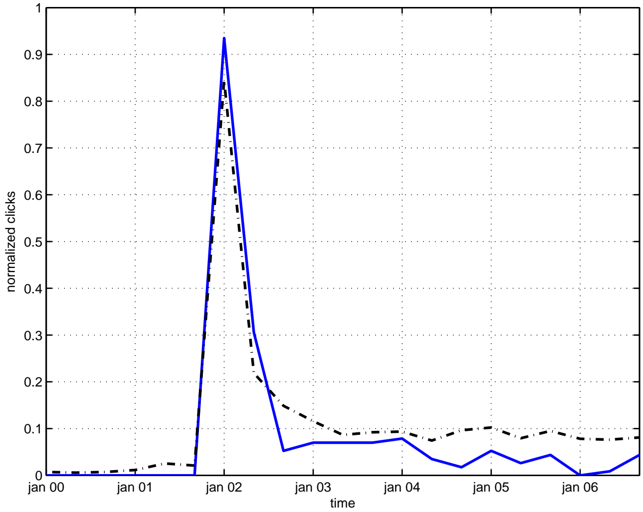
spontaneously broken r parity
