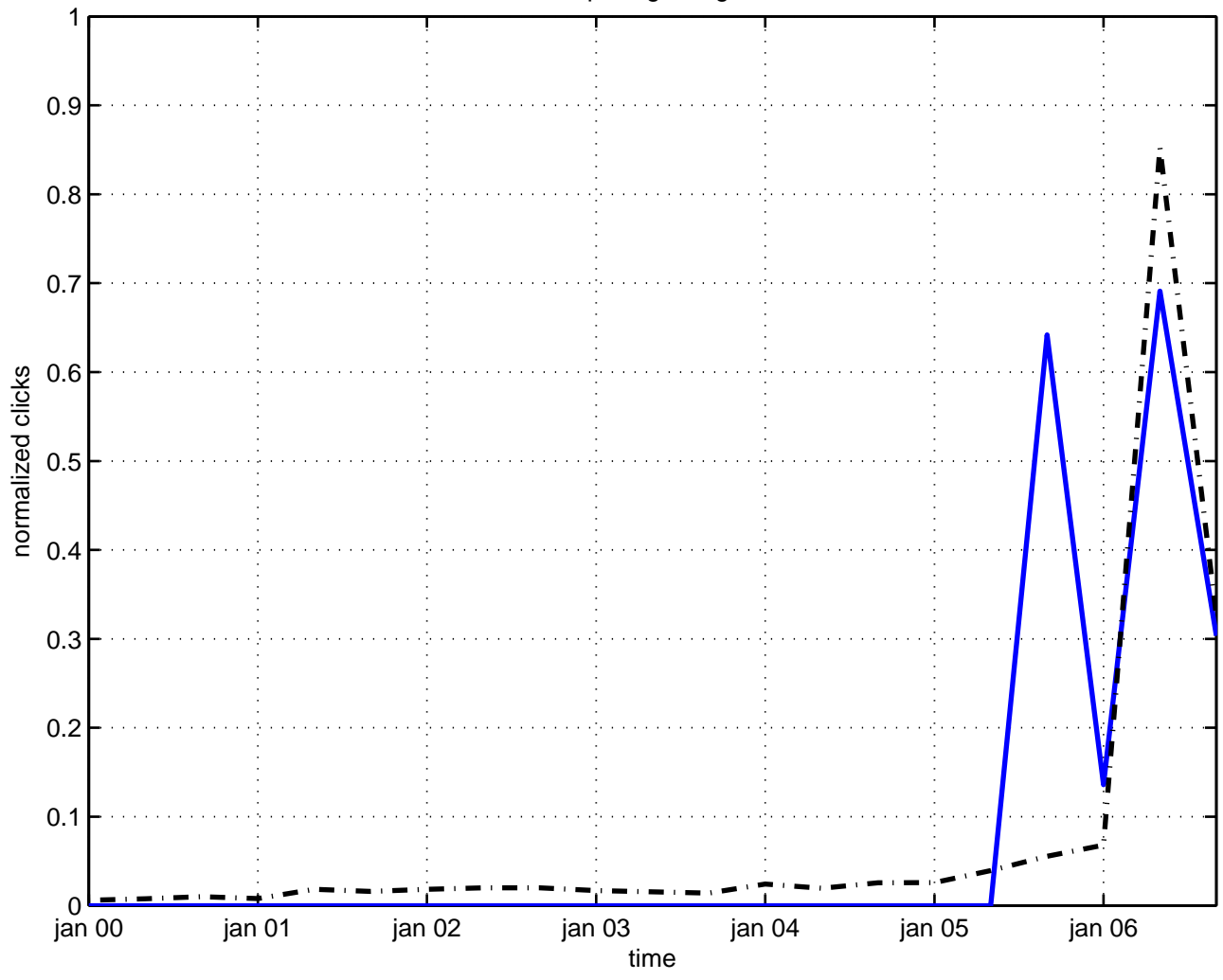
splitting string
