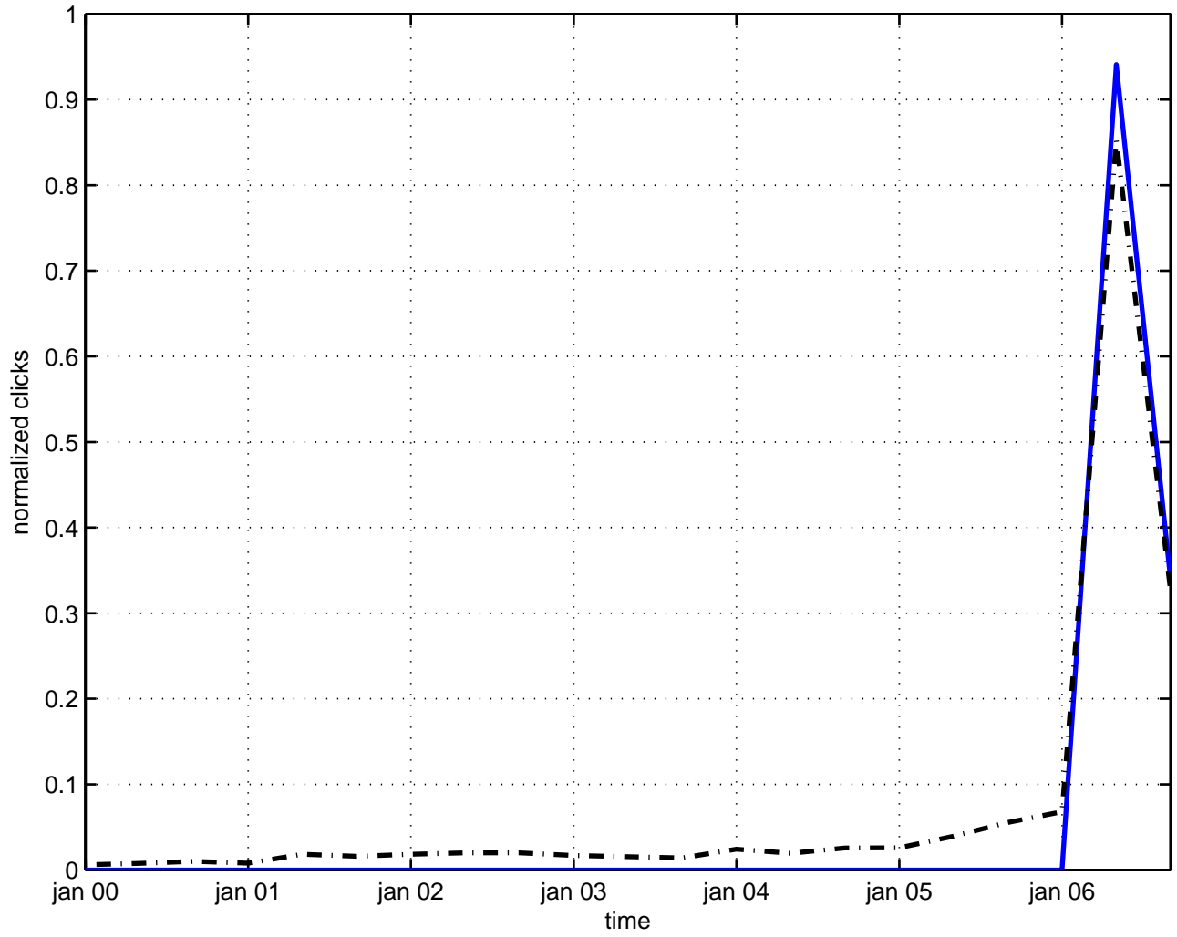
split octonion
