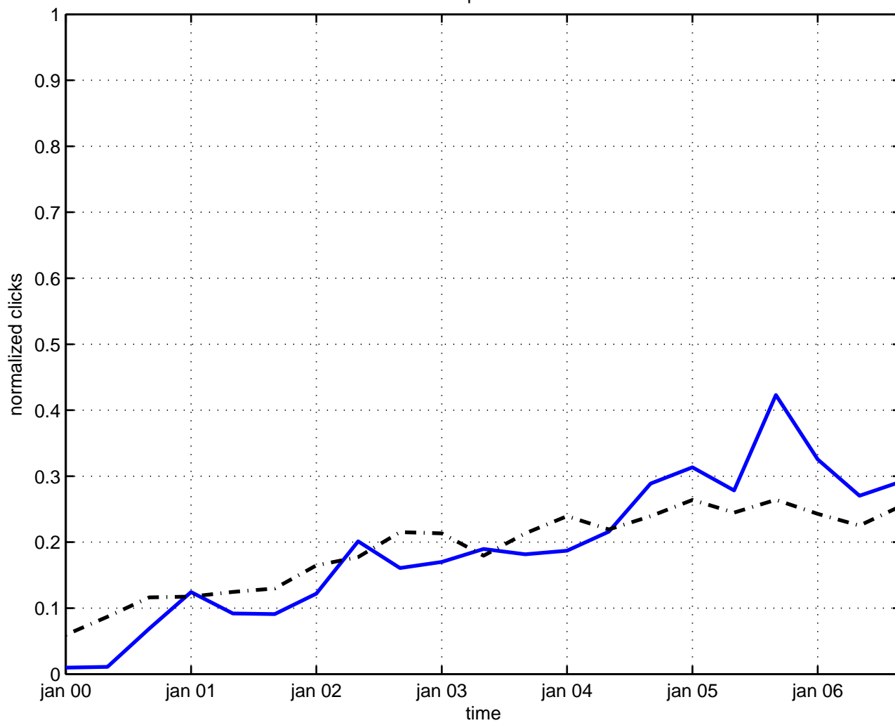
spinor
