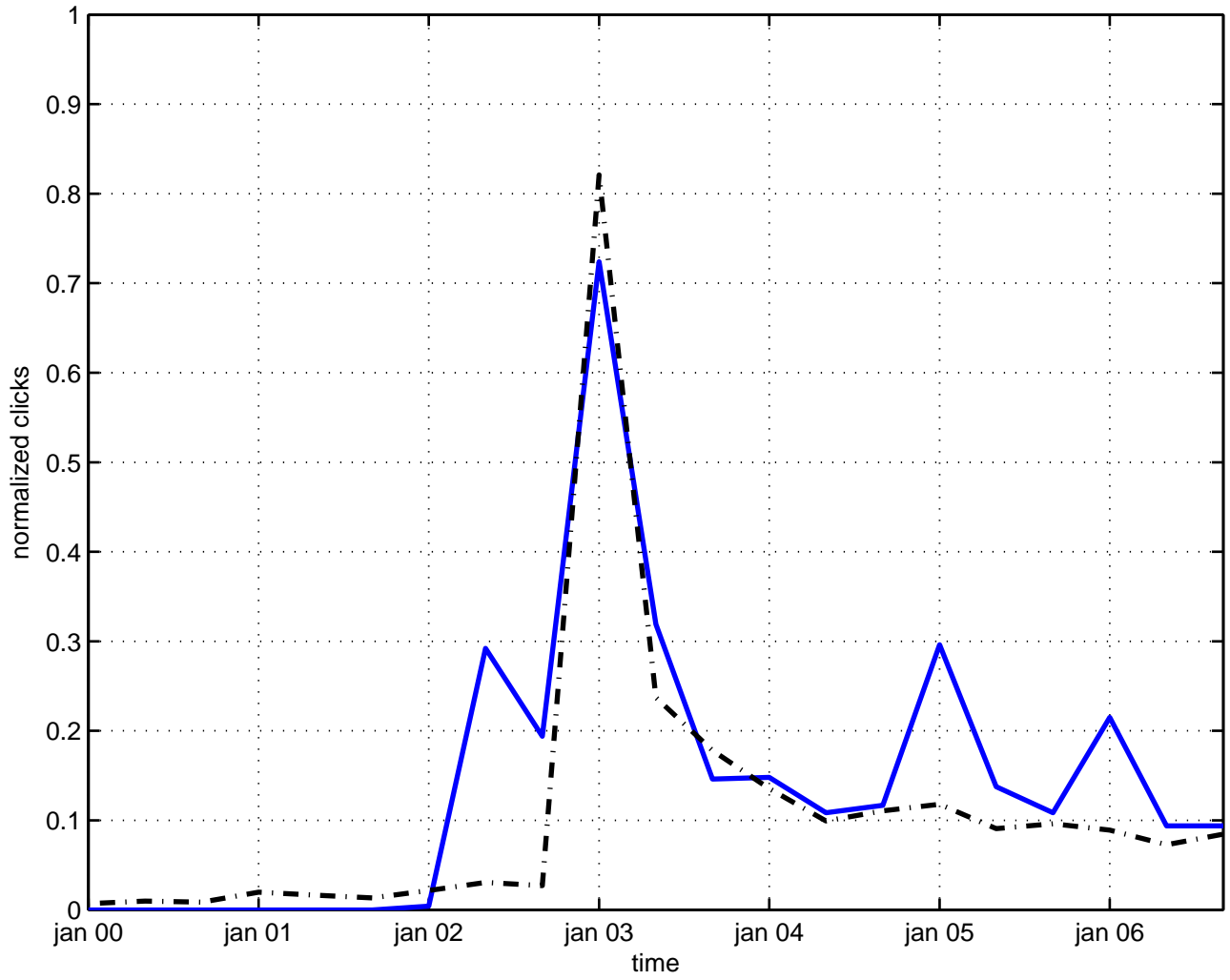
spinor quantum electrodynamics
