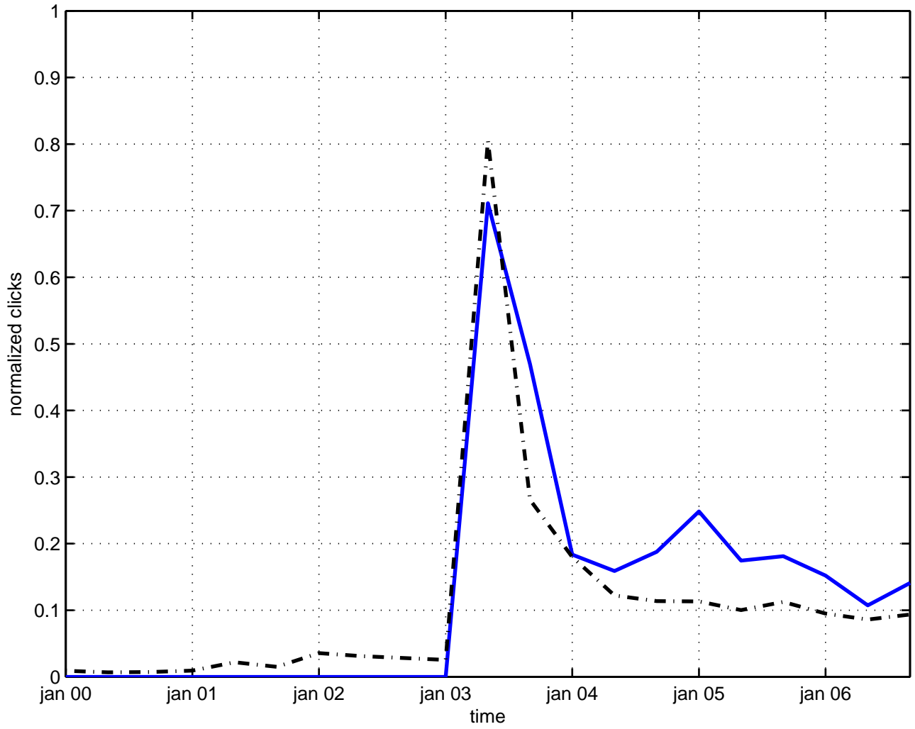
spinor model
