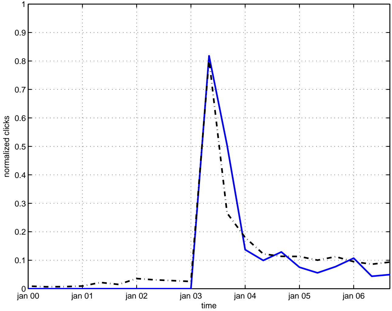
spinor gravitation
