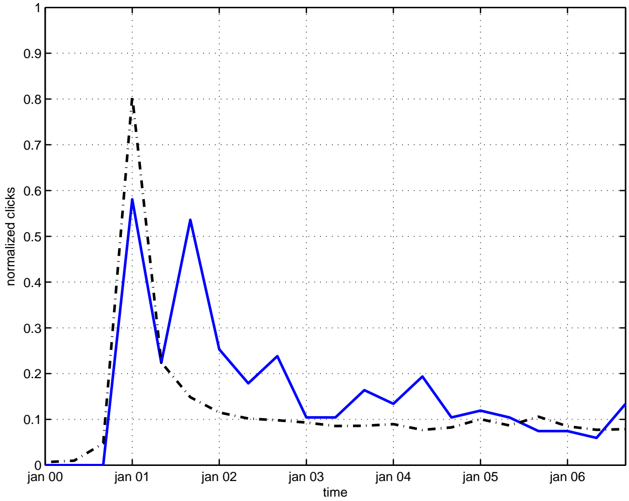
spinless bethe-salpeter equation
