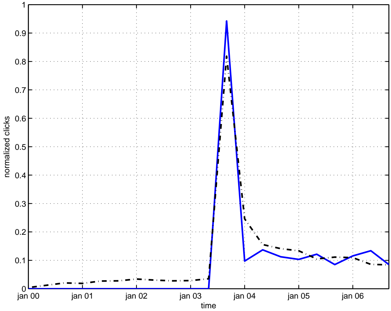
spin hadron
