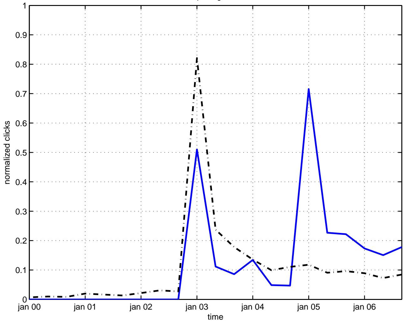
spin algebra
