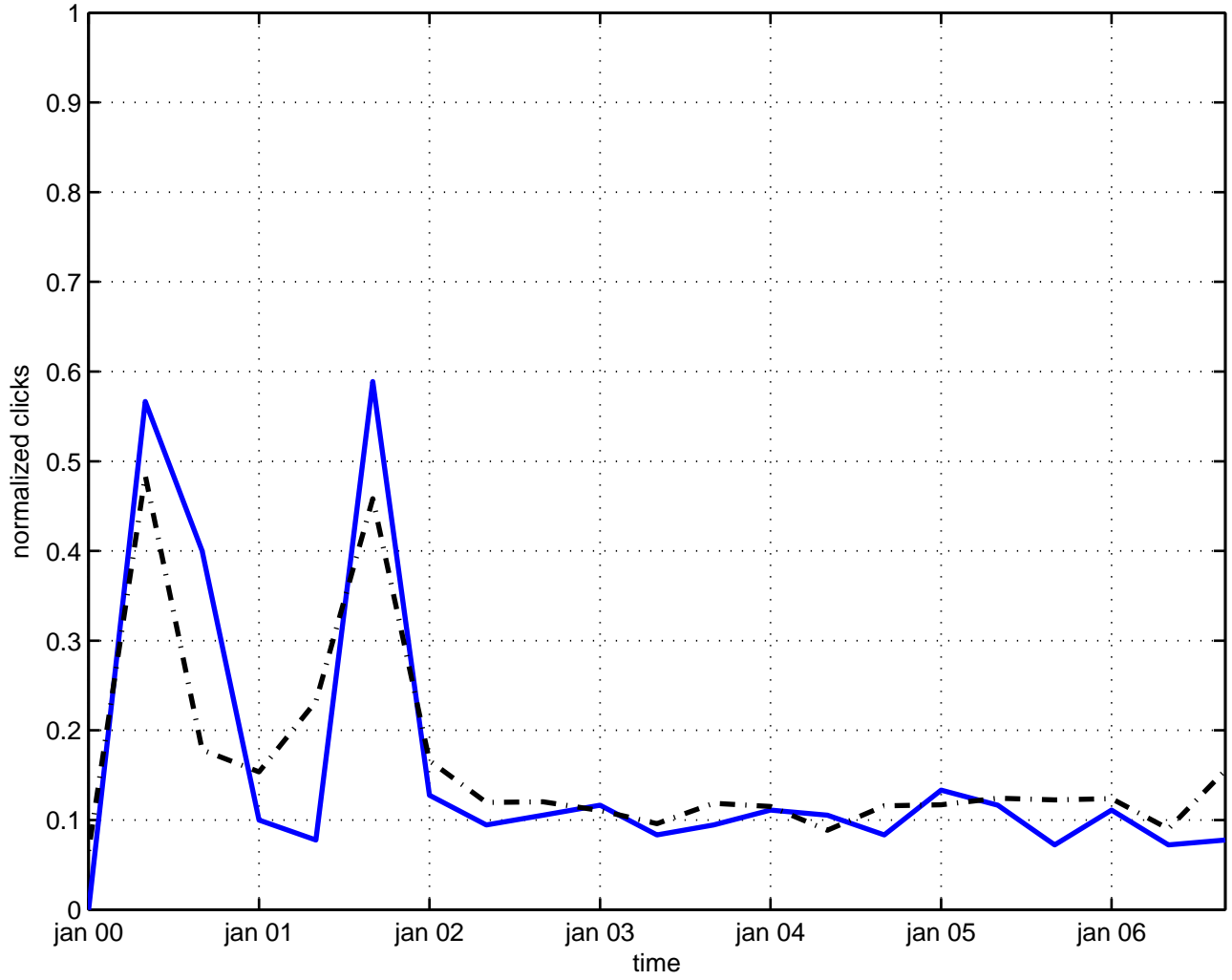
spin(n) group theory
