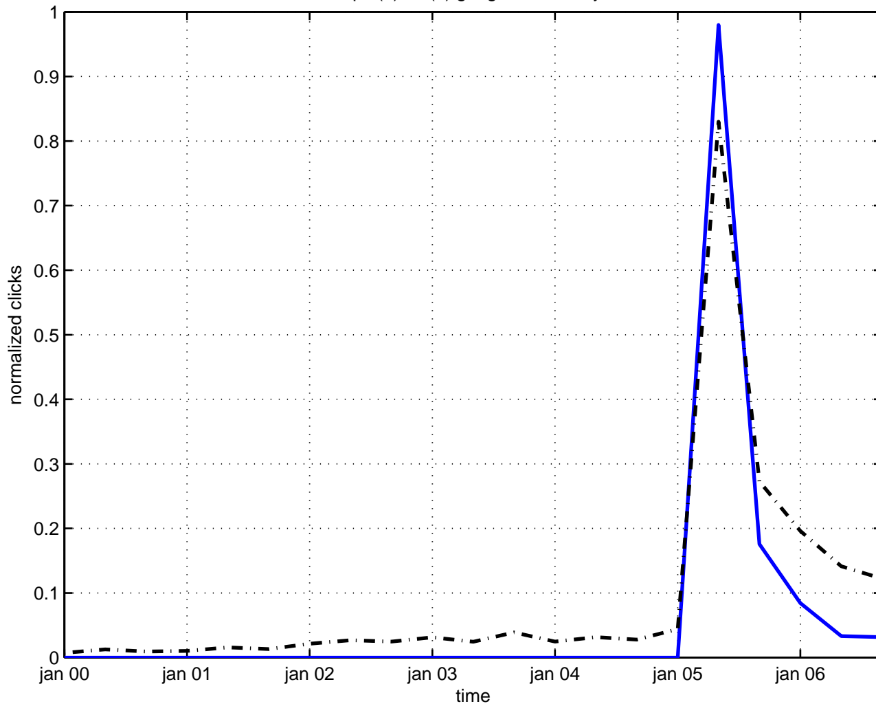
spin(8) x e(8) gauge field theory
