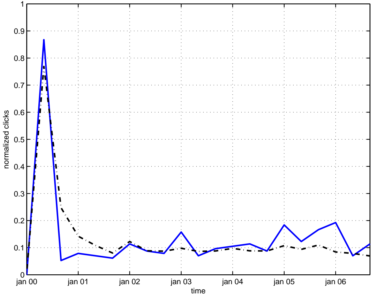
spin(8) group theory
