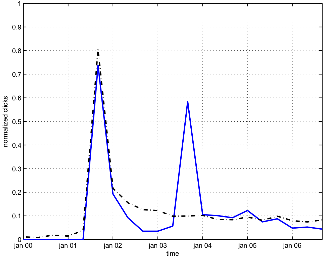
spin(7) invariance
