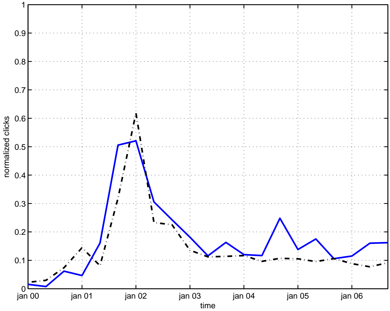
spin(7) holonomy
