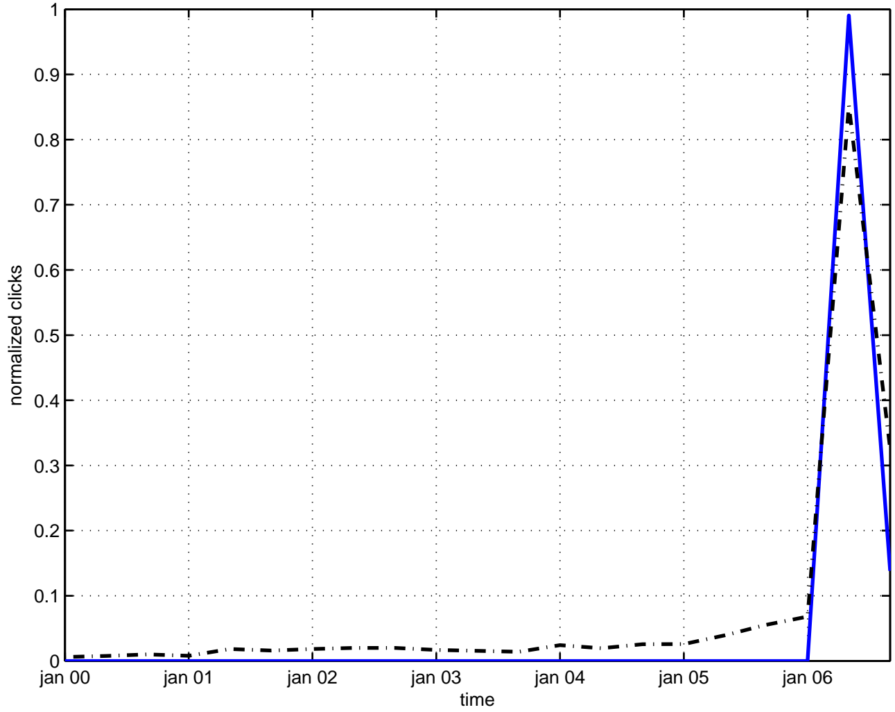
spin(32)/z(2) gauge field theory
